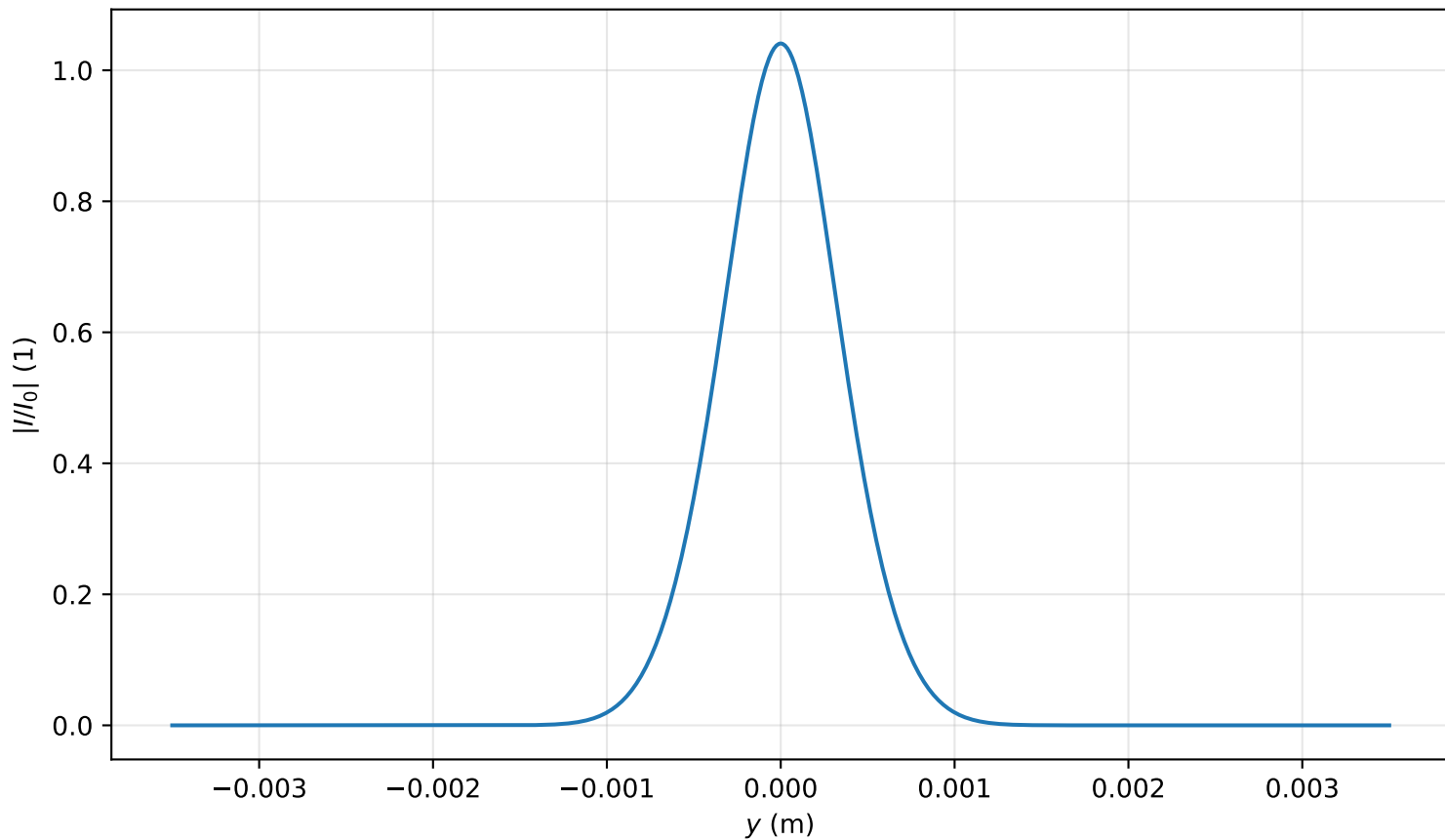
Intensity profile I(x=0, y, z=0.478)/I_0 , P_{in}=0.5P_{cr} , artificial time
